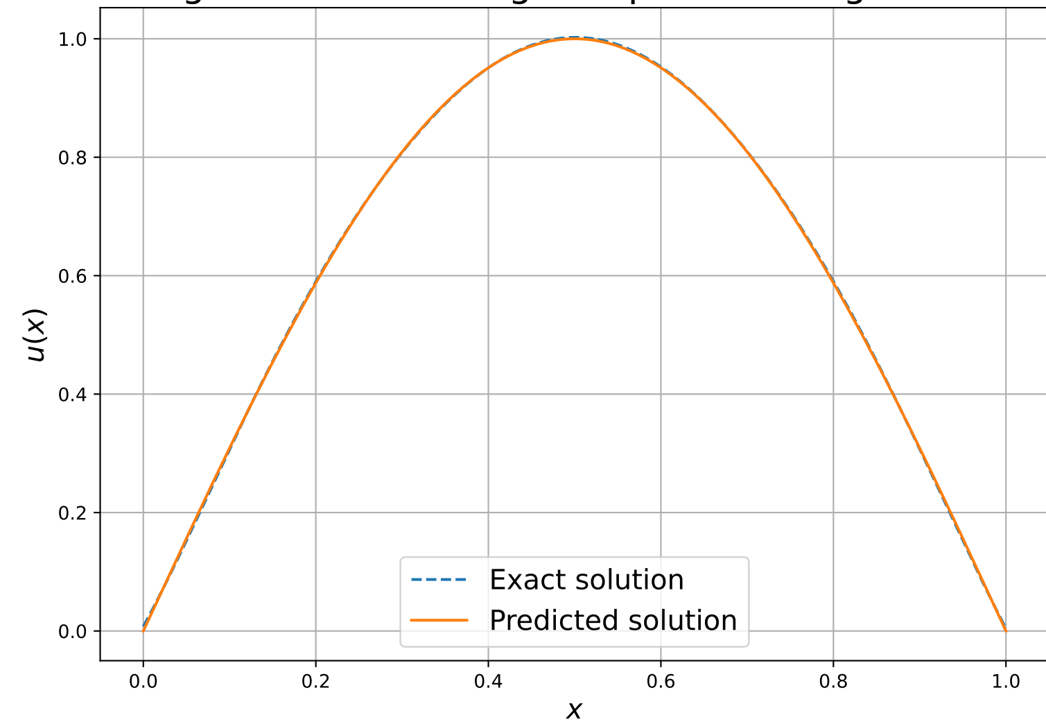
Solving 1D Volterra integral equation using MC-cPIKAN
